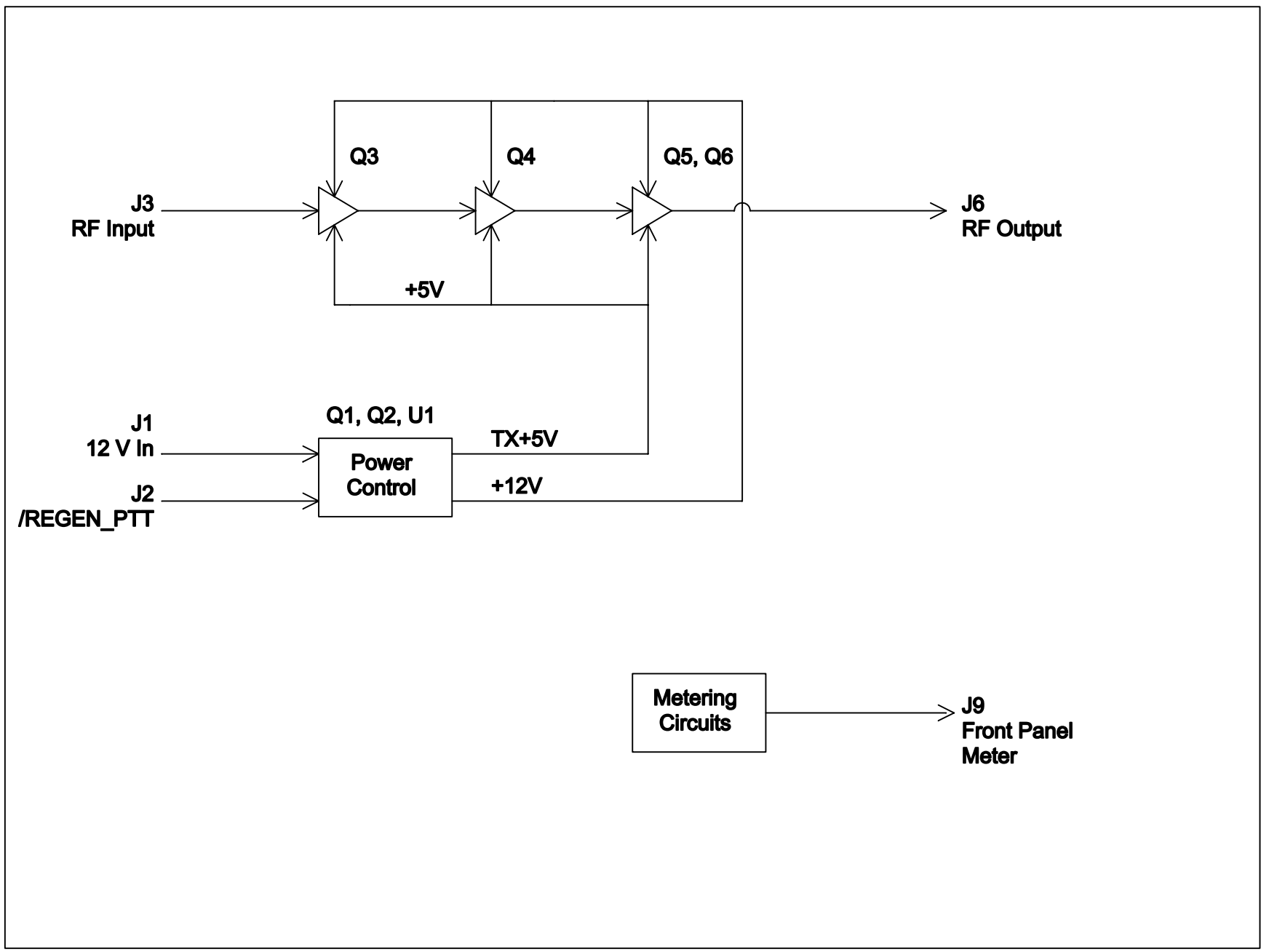
RF Power Amplifier Block Diagram Sheet 1
