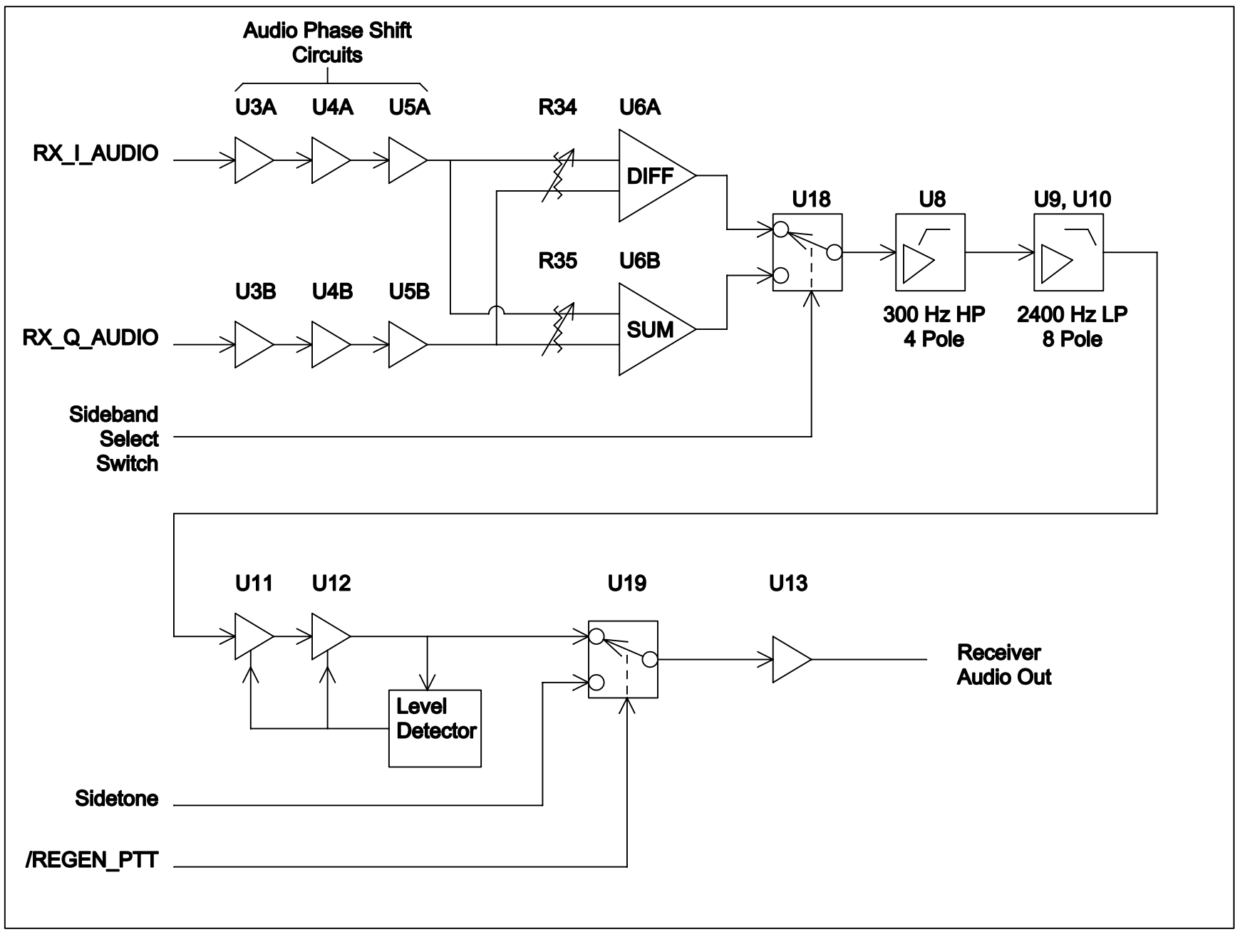
Receiver Block Diagram Sheet 2
