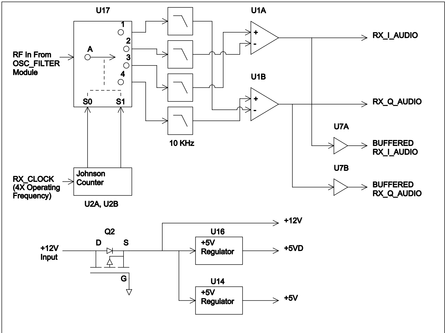
Receiver Block Diagram Sheet 1
