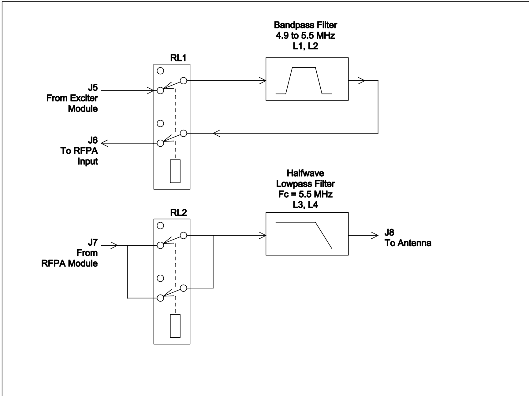
Oscillator-Filter Transmit Path Block Diagram Sheet 1
