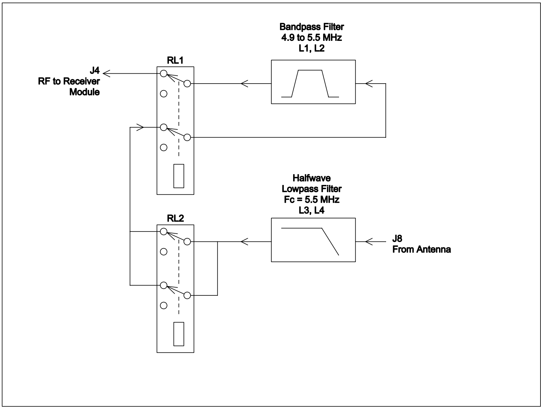
Oscillator-Filter Receive RF Path Block Diagram Sheet 1
