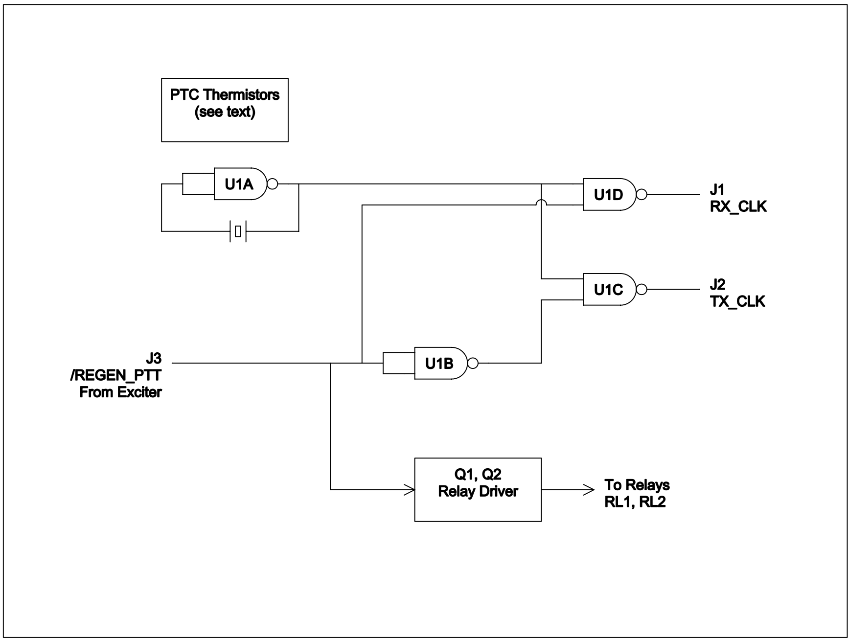
Oscillator-Filter Clock Block Diagram Sheet 1
