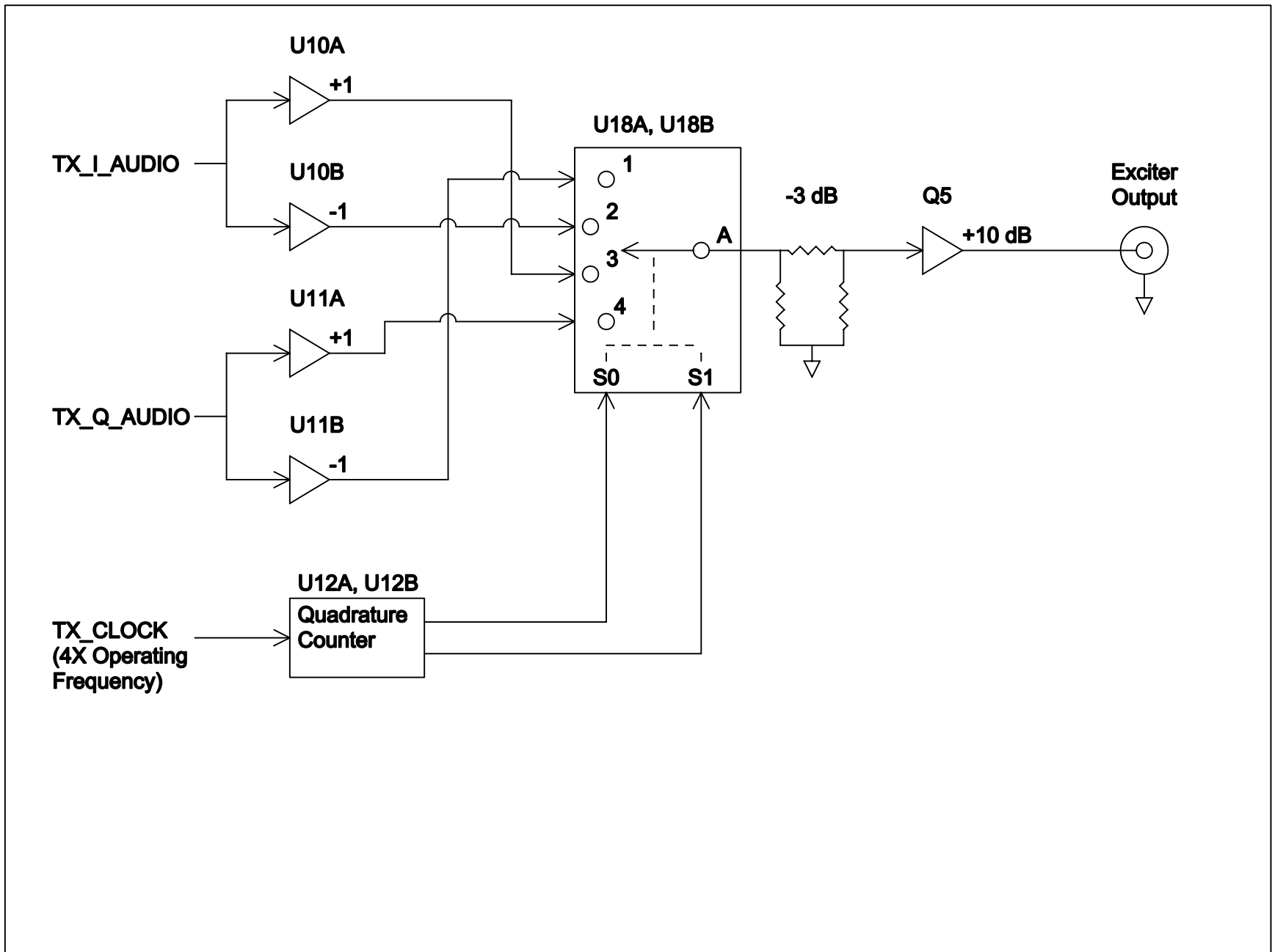
Exciter Block Diagram Sheet 3
