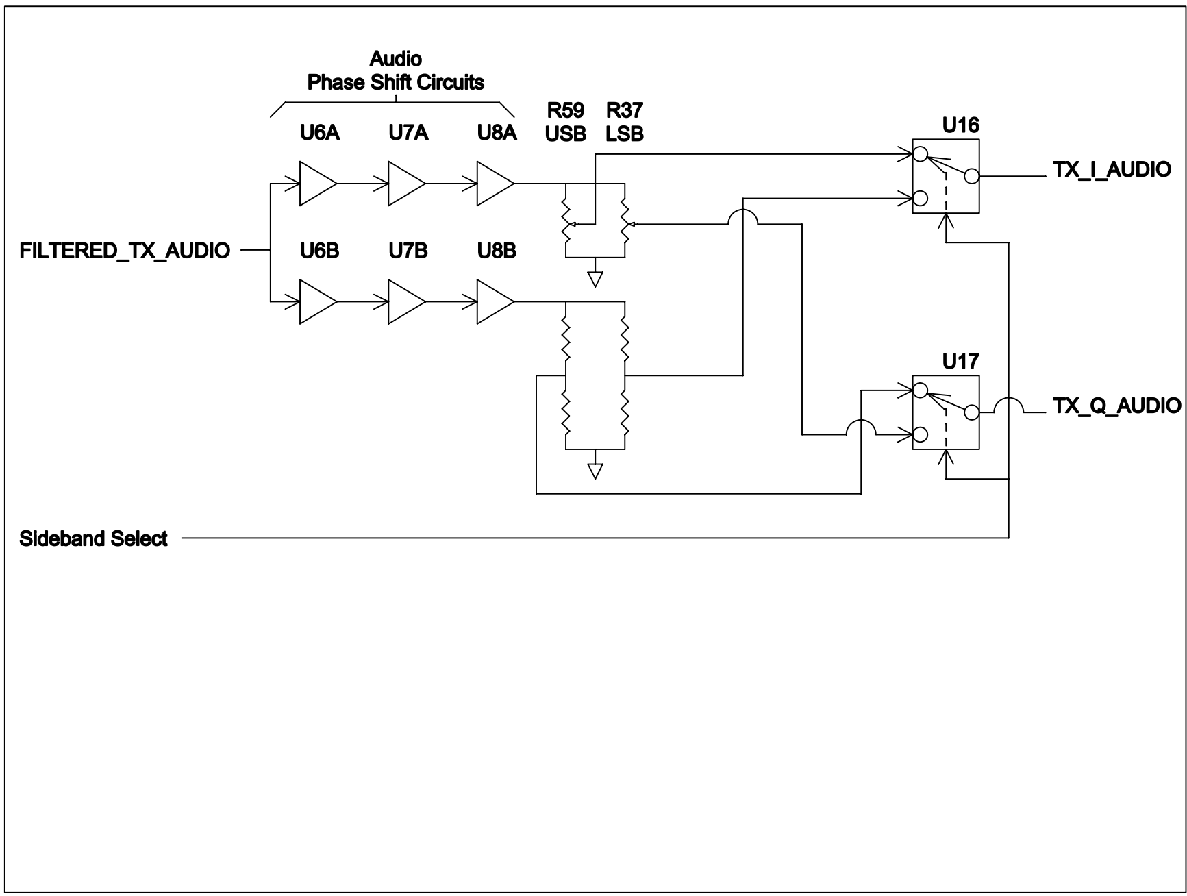
Exciter Block Diagram Sheet 2
