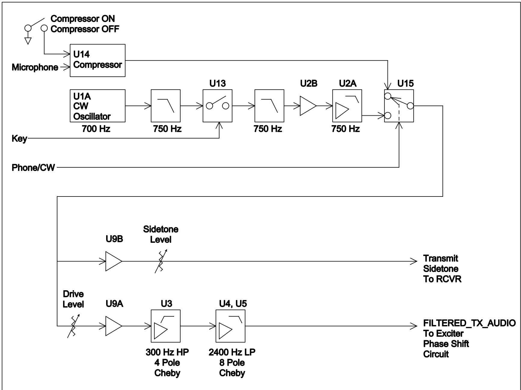
Exciter Block Diagram Sheet 1
